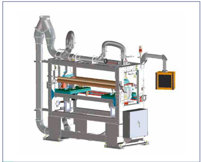
Edge trimming saw with 2 units for edge cutting.
